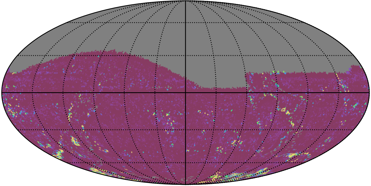
ddf_acor_sf15_lsf40_lsr50_v3.4_10yrs All sky g band: 75th Percentile Intranight Timespan
