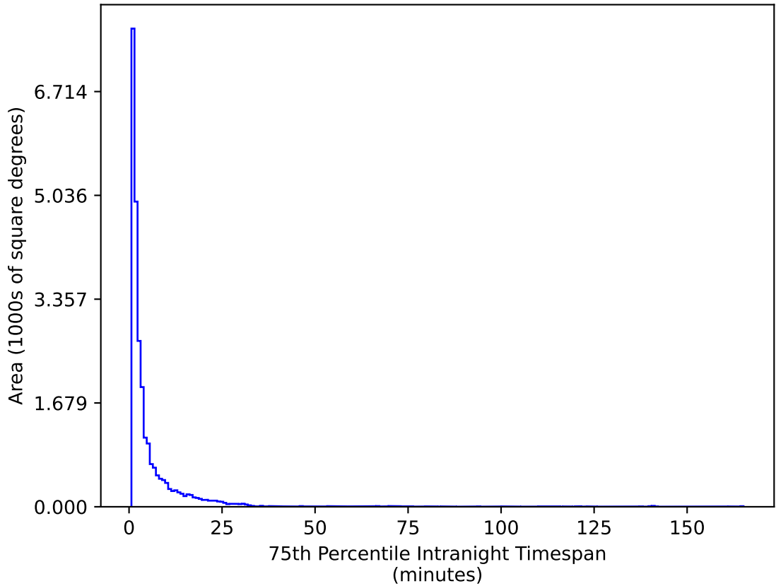
ddf_acor_sf15_lsf40_lsr50_v3.4_10yrs All sky g band: 75th Percentile Intranight Timespan
