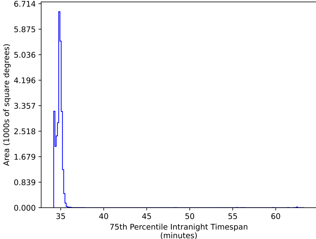
ddf_acor_sf15_lsf40_lsr50_v3.4_10yrs All sky all bands: 75th Percentile Intranight Timespan
