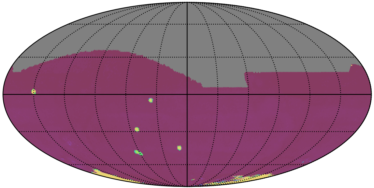
ddf_acor_sf15_lsf40_lsr50_v3.4_10yrs All sky: 75th Percentile Intranight Timespan
