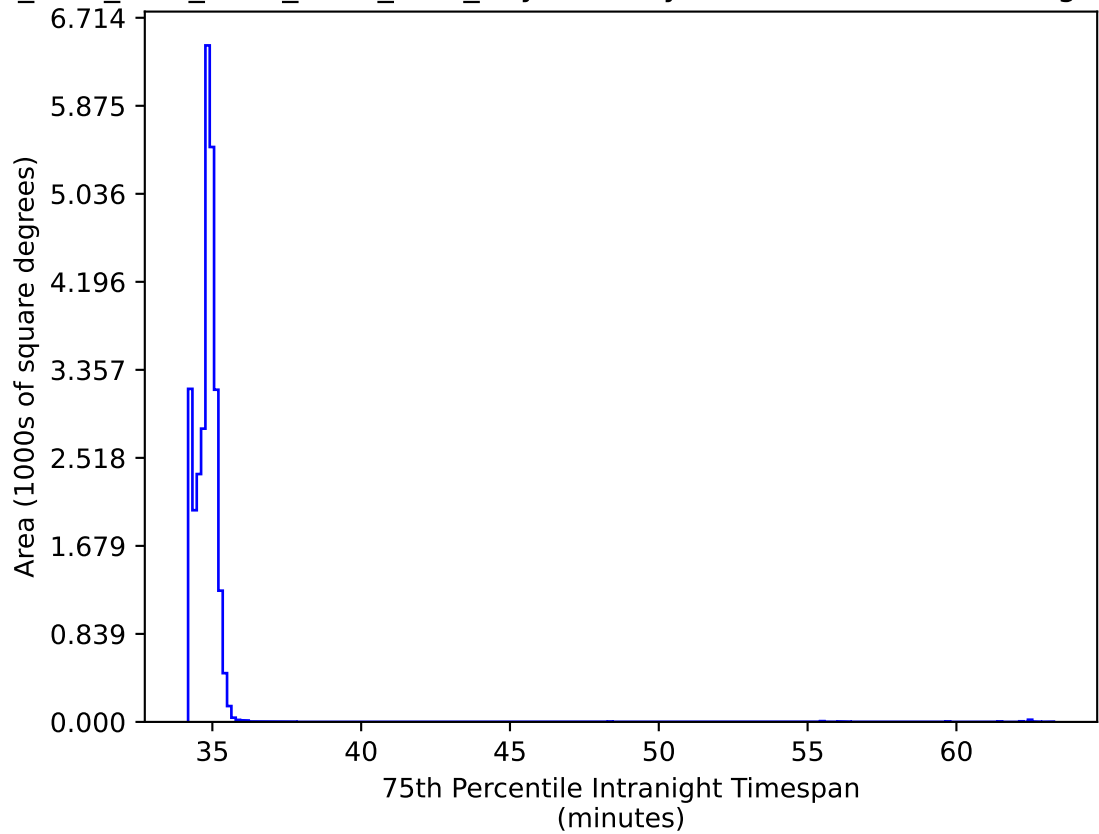
ddf_acor_sf15_lsf40_lsr50_v3.4_10yrs All sky: 75th Percentile Intranight Timespan
