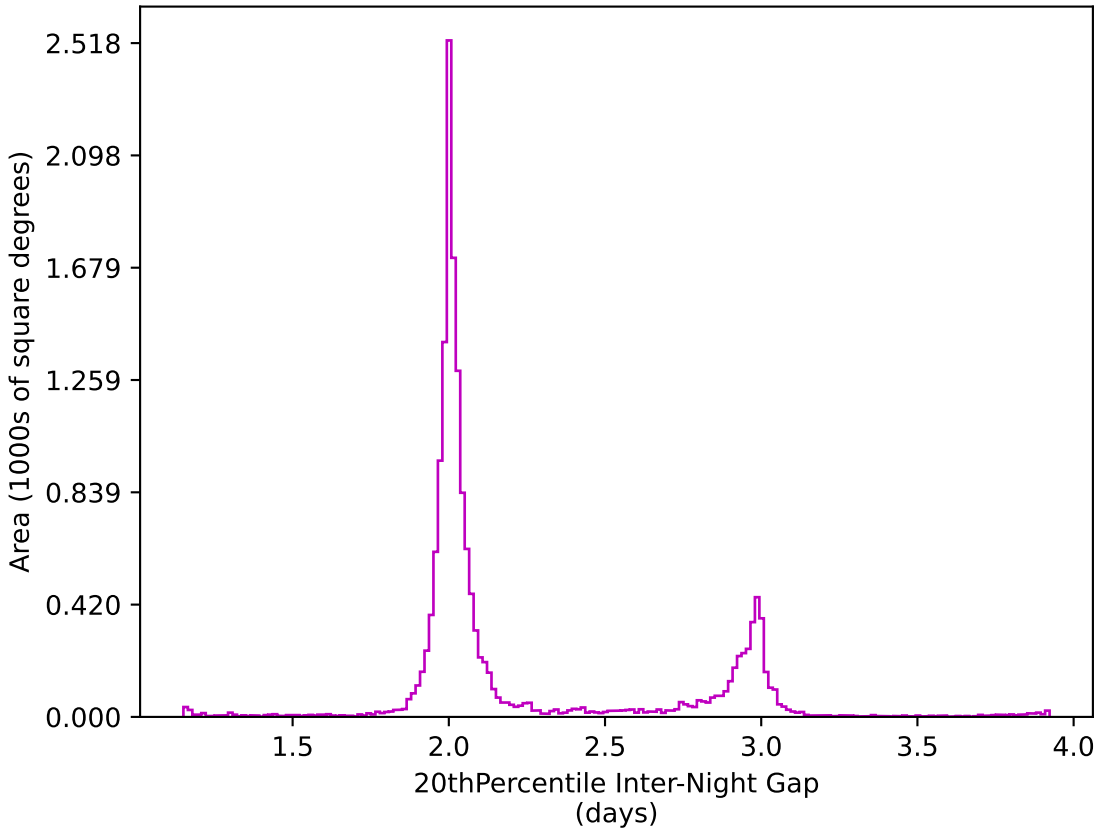
ddf_acor_sf15_lsf40_lsr50_v3.4_10yrs WFD z band: 20thPercentile Inter-Night Gap
