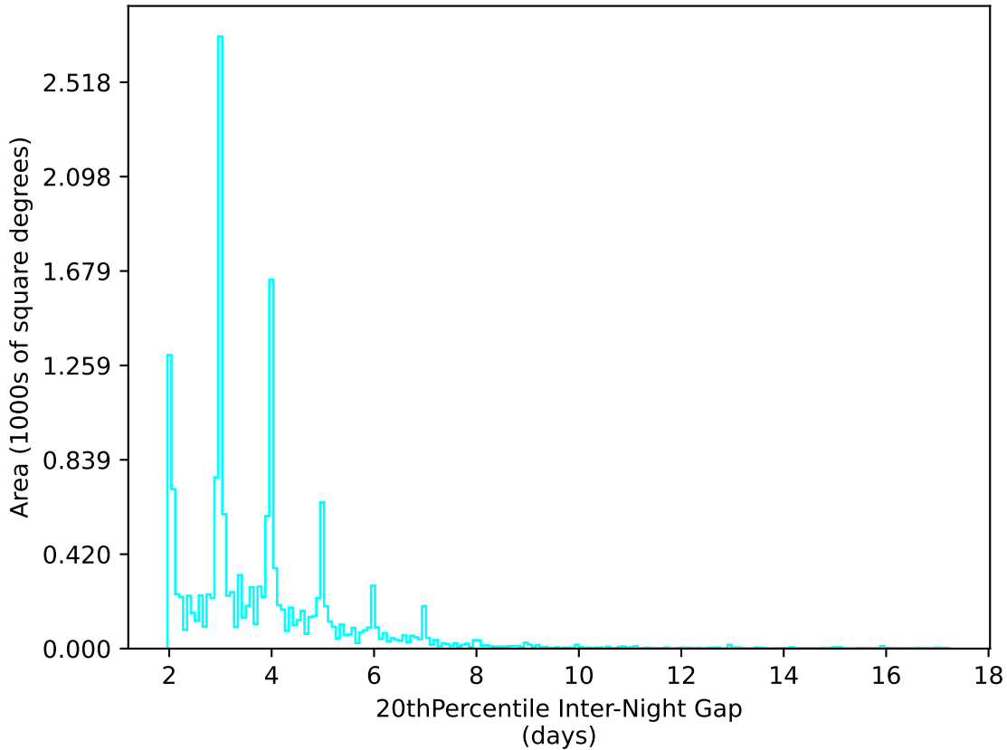
ddf_acor_sf15_lsf40_lsr50_v3.4_10yrs WFD u band: 20thPercentile Inter-Night Gap
