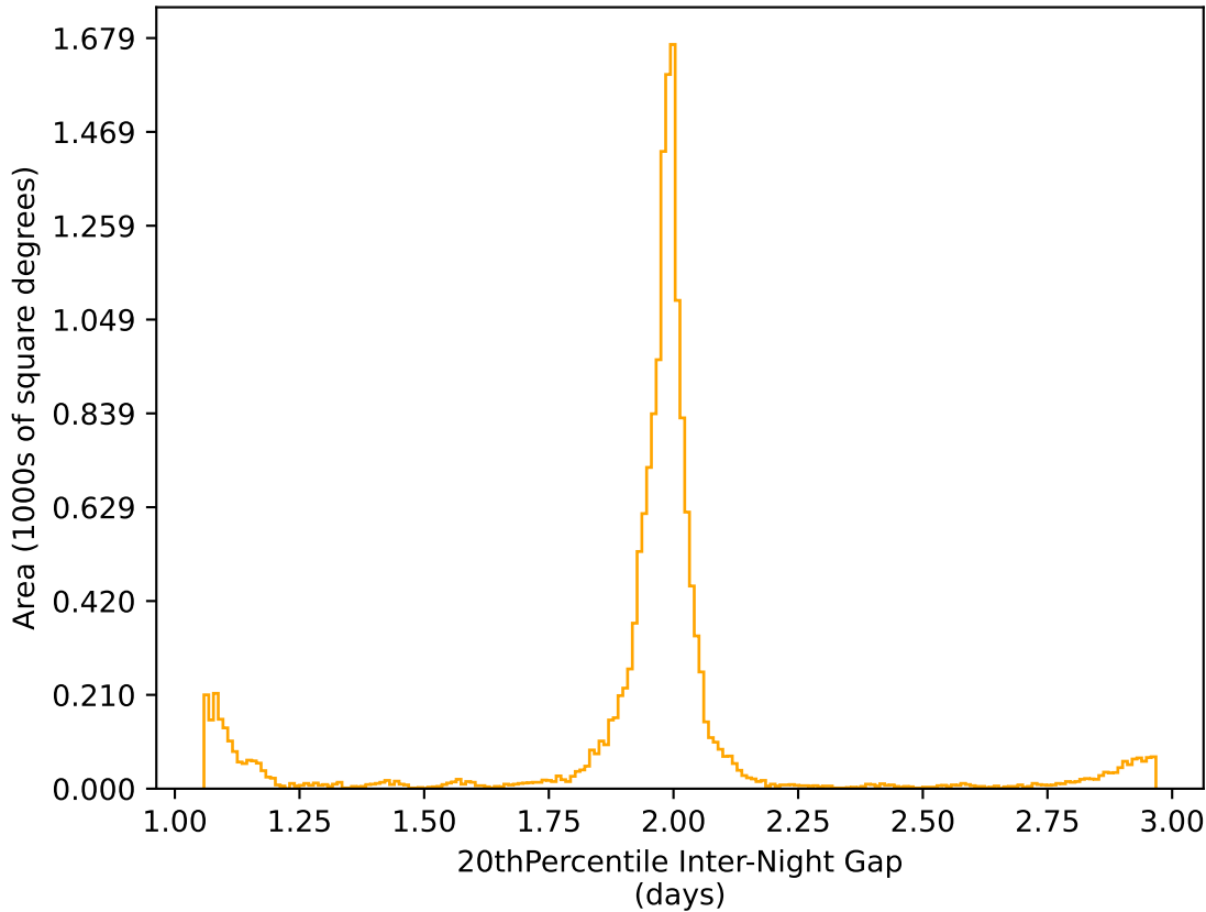
ddf_acor_sf15_lsf40_lsr50_v3.4_10yrs WFD r band: 20thPercentile Inter-Night Gap
