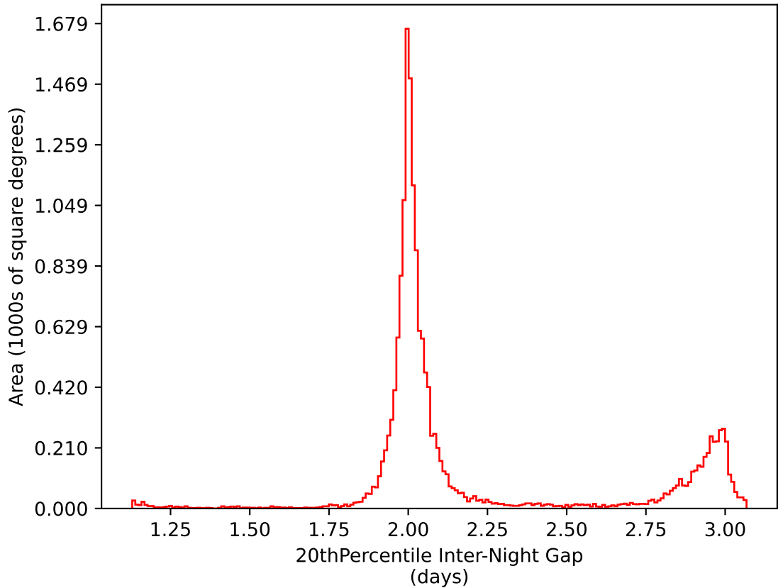
ddf_acor_sf15_lsf40_lsr50_v3.4_10yrs WFD i band: 20thPercentile Inter-Night Gap
