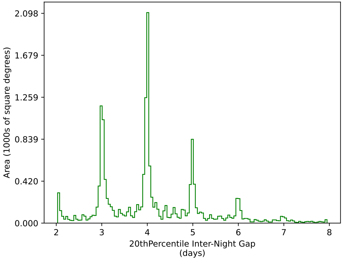
ddf_acor_sf15_lsf40_lsr50_v3.4_10yrs WFD g band: 20thPercentile Inter-Night Gap
