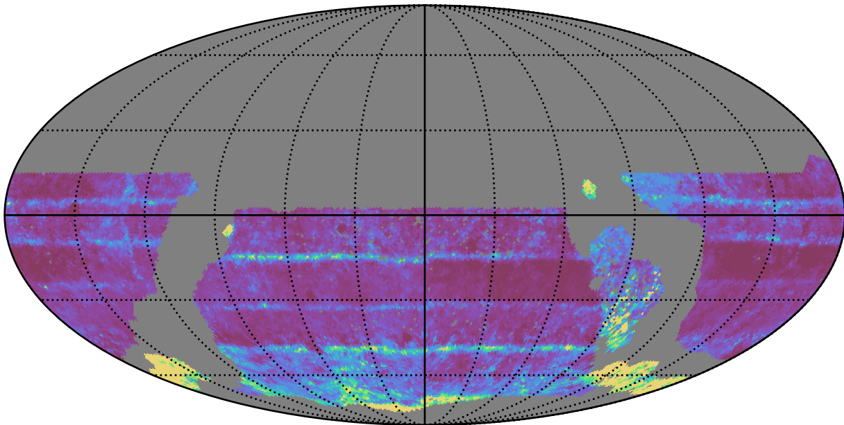
ddf_acor_sf15_lsf40_lsr50_v3.4_10yrs WFD all bands: 20thPercentile Inter-Night Gap
