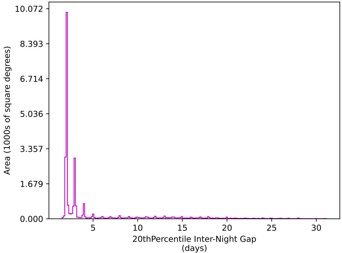
ddf_acor_sf15_ls40_lsr50_v3.4_10yrs All sky z band: 20thPercentile Inter-Night Gap
