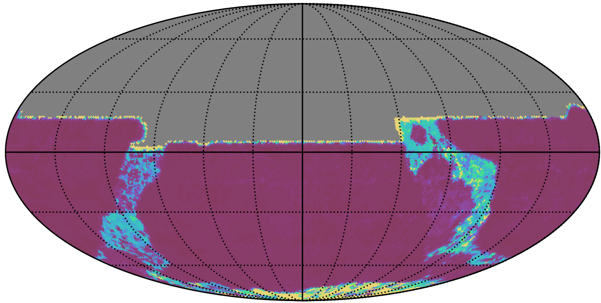
ddf_acor_sf15_lsf40_lsr50_v3.4_10yrs All sky y band: 20thPercentile Inter-Night Gap
