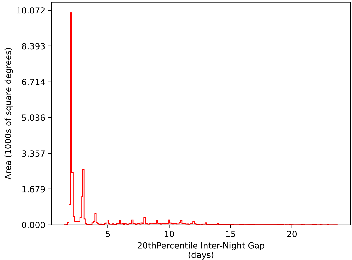
ddf_acor_sf15_lsf40_lsr50_v3.4_10yrs All sky i band: 20thPercentile Inter-Night Gap
