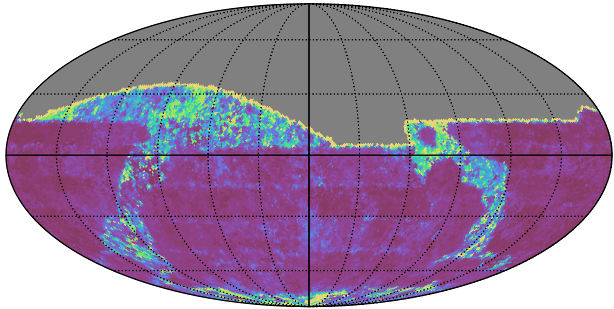
ddf_acor_sf15_lsf40_lsr50_v3.4_10yrs All sky g band: 20thPercentile Inter-Night Gap
