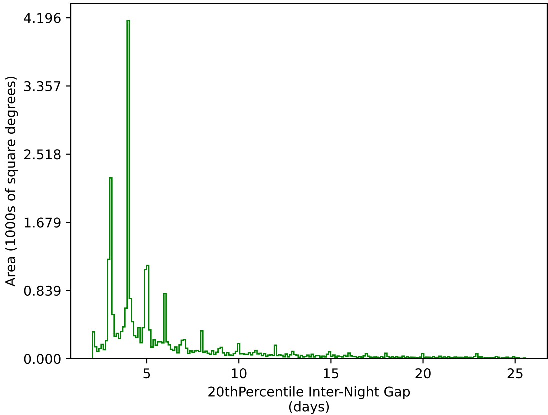
ddf_acor_sf15_ls40_lsr50_v3.4_10yrs All sky g band: 20thPercentile Inter-Night Gap
