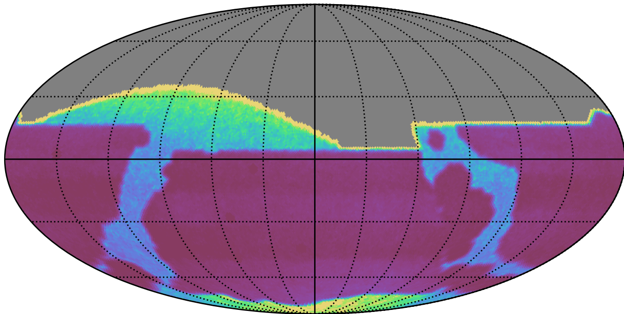
ddf_acor_sf15_lsf40_lsr50_v3.4_10yrs : properMotion
