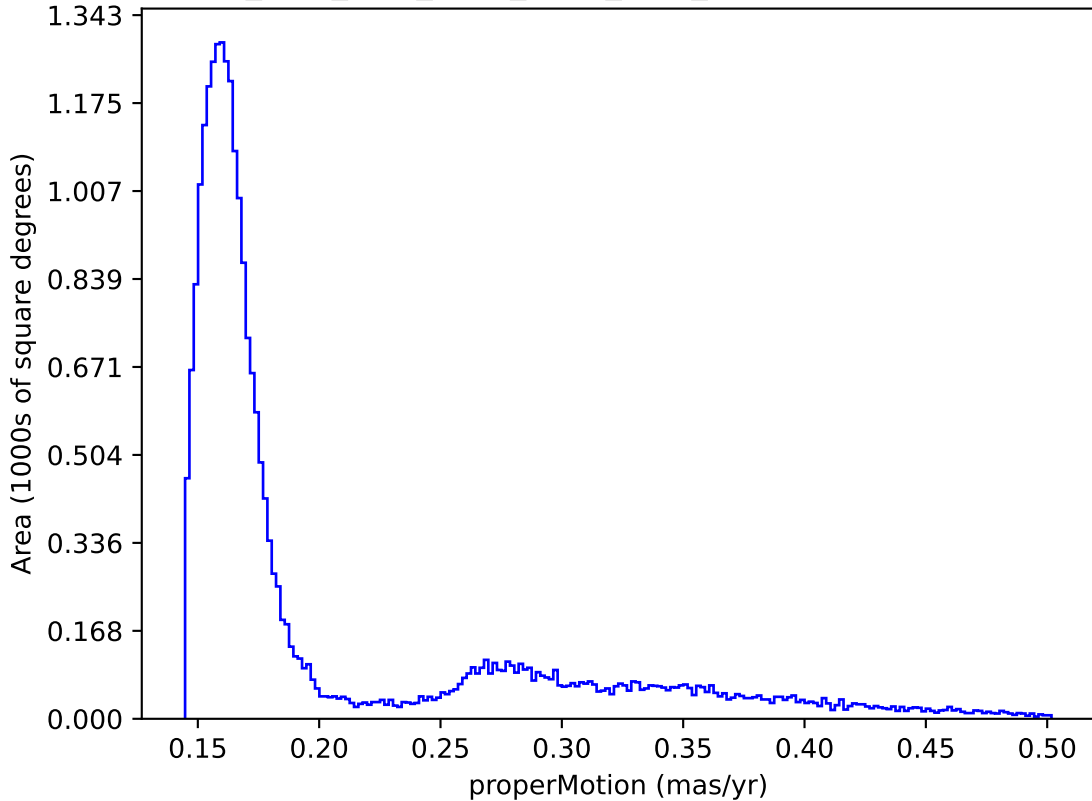
ddf_acor_sf15_lsf40_lsr50_v3.4_10yrs : properMotion
