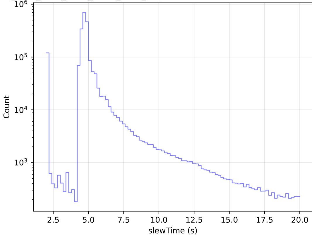
ddf_acor_sf15_Isf40_Isr50_v3.4_10yrs All visits: Zoom Slew Time Histogram
