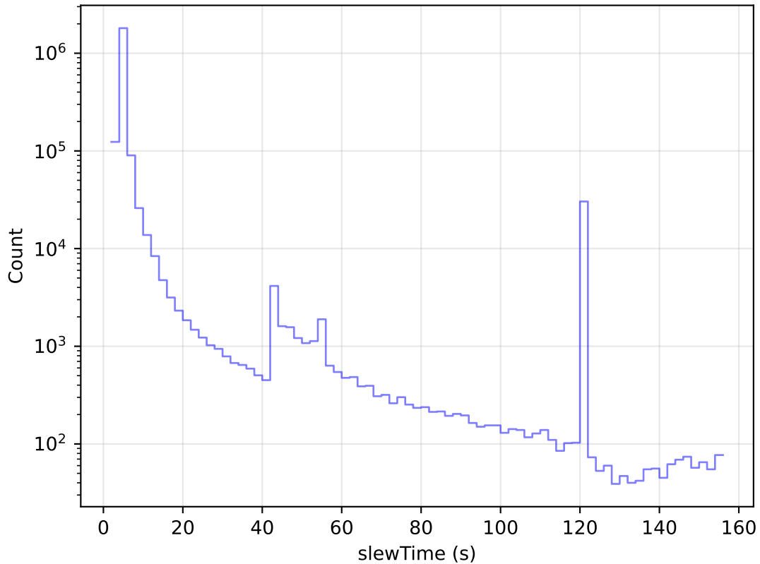
ddf_acor_sf15_lsf40_lsr50_v3.4_10yrs All visits: Slew Time Histogram
