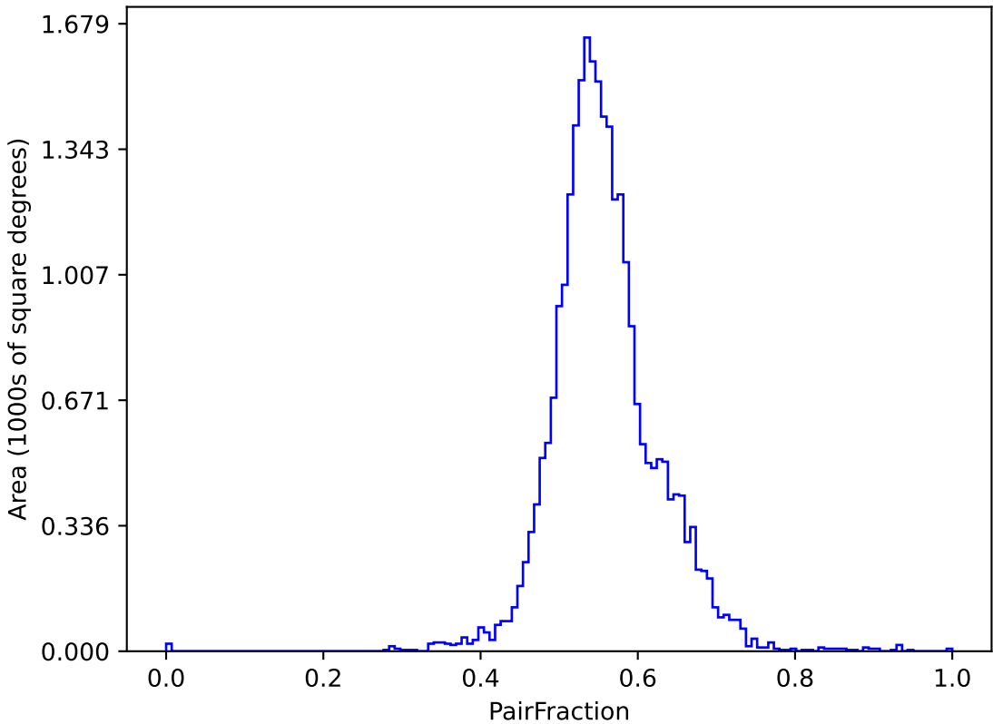
ddf_acor_sf15_lsf40_lsr50_v3.4_10yrs (g or r or i): PairFraction
