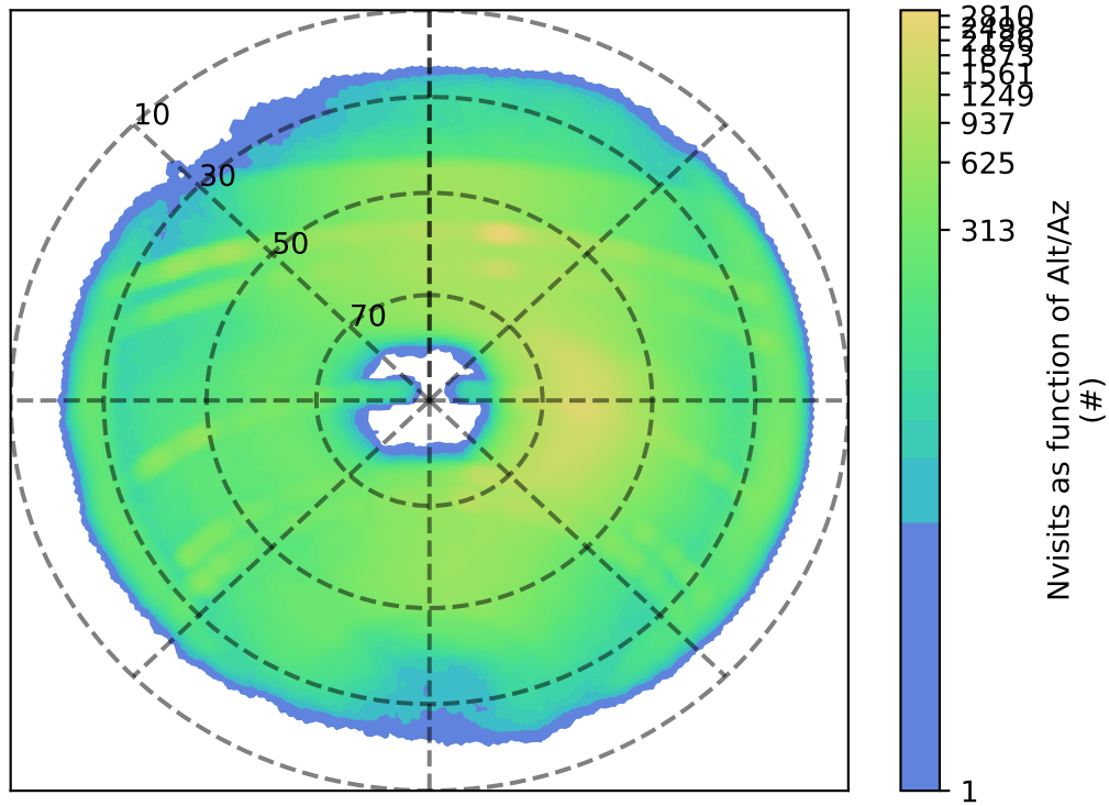
ddf_acor_sf15_lsf40_lsr50_v3.4_10yrs z: Nvisits as function of Alt/Az
