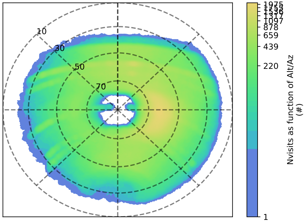
ddf_acor_sf15_lsf40_lsr50_v3.4_10yrs y: Nvisits as function of Alt/Az
