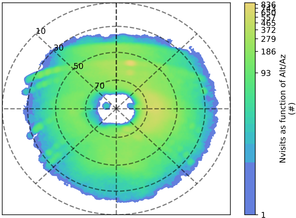
ddf_acor_sf15_lsf40_lsr50_v3.4_10yrs u: Nvisits as function of Alt/Az
