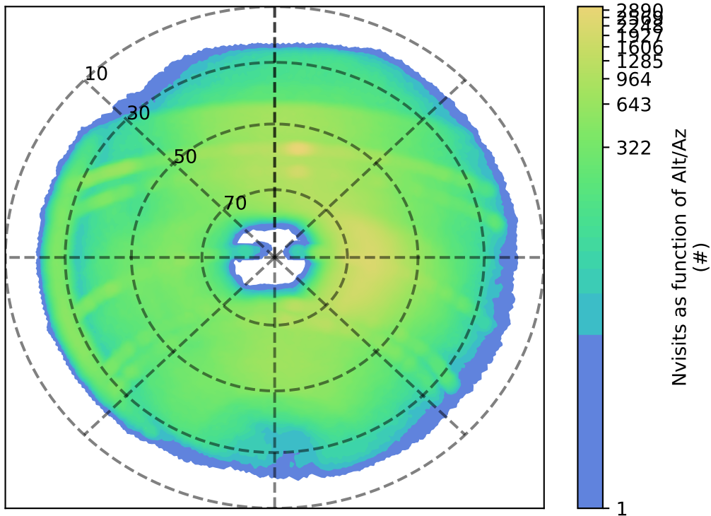
ddf_acor_sf15_ls40_lsr50_v3.4_10yrs r: Nvisits as function of Alt/Az
