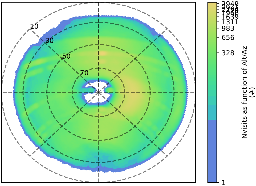
ddf_acor_sf15_ls40_lsr50_v3.4_10yrs i: Nvisits as function of Alt/Az
