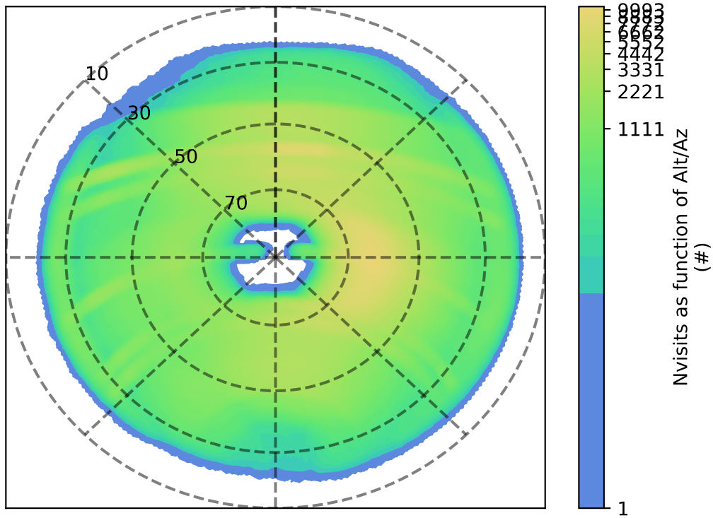
ddf_acor_sf15_lsf40_lsr50_v3.4_10yrs : Nvisits as function of Alt/Az
