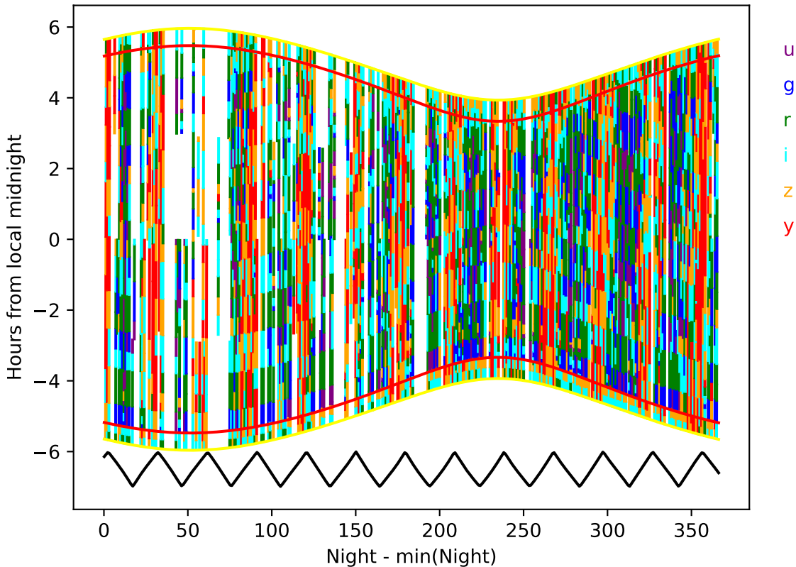
ddf_acor_sf15_lsf40_lsr50_v3.4_10yrs year 9-10: Hourglass
