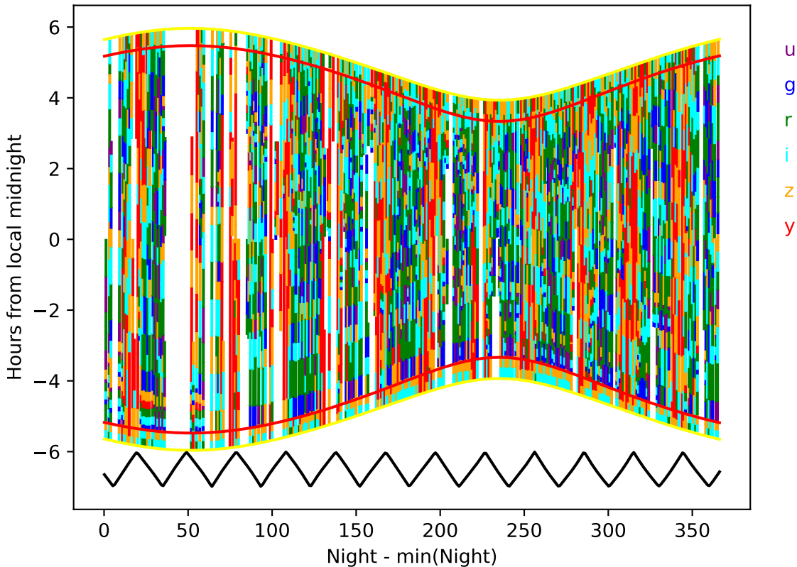
ddf_acor_sf15_lsf40_lsr50_v3.4_10yrs year 2-3: Hourglass
