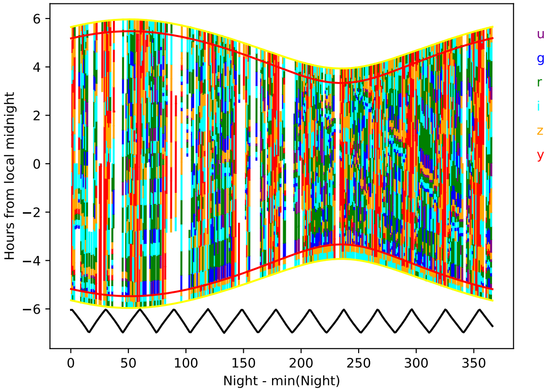
ddf_acor_sf15_lsf40_lsr50_v3.4_10yrs year 1-2: Hourglass
