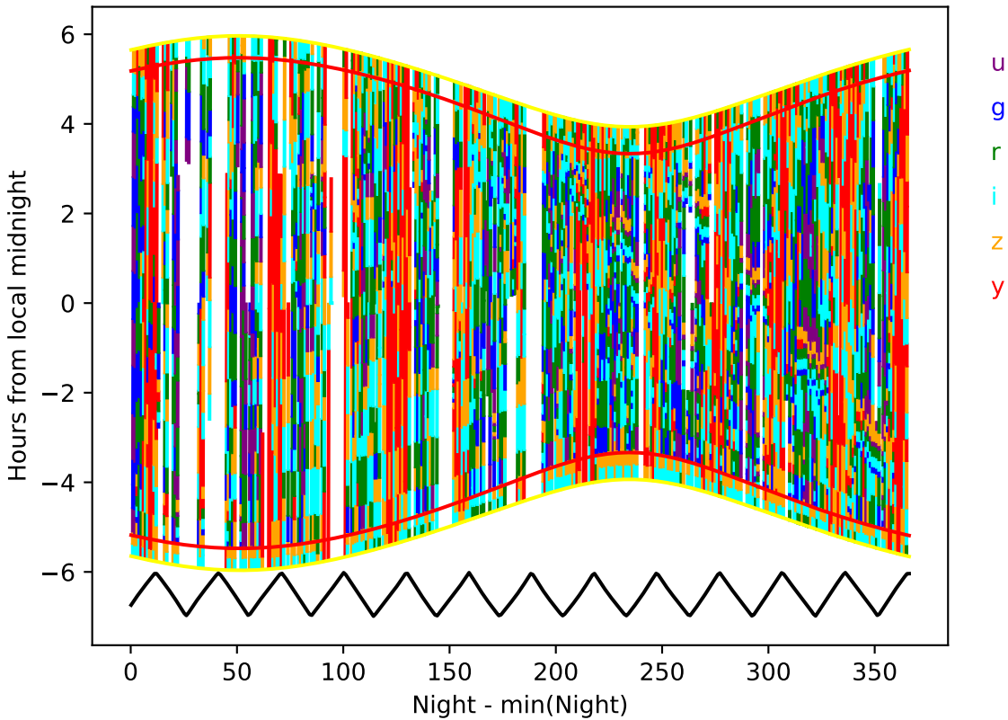
ddf_acor_sf15_lsf40_lsr50_v3.4_10yrs year 0-1: Hourglass
