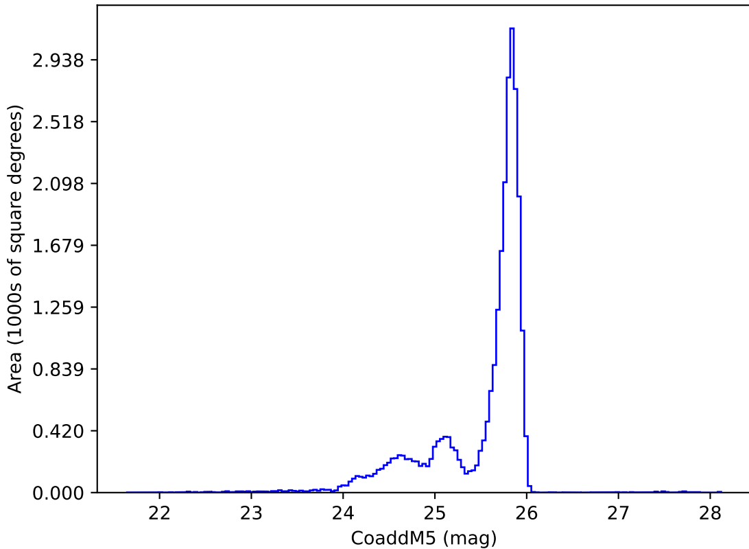
ddf_acor_sf15_lsf40_lsr50_v3.4_10yrs z: CoaddM5
