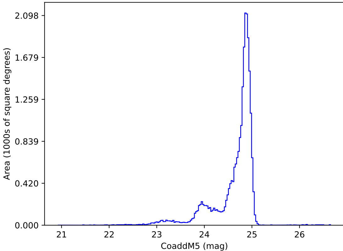
ddf_acor_sf15_lsf40_lsr50_v3.4_10yrs y: CoaddM5
