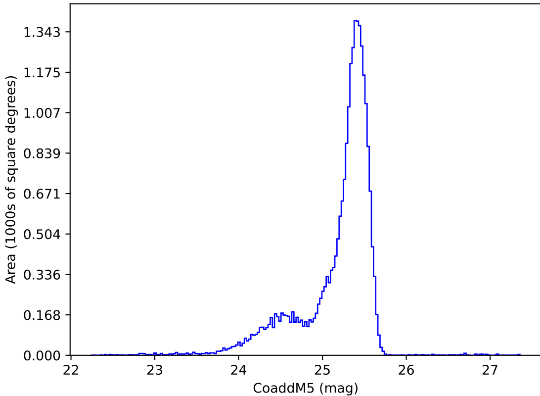
ddf_acor_sf15_ls40_lsr50_v3.4_10yrs u: CoaddM5
