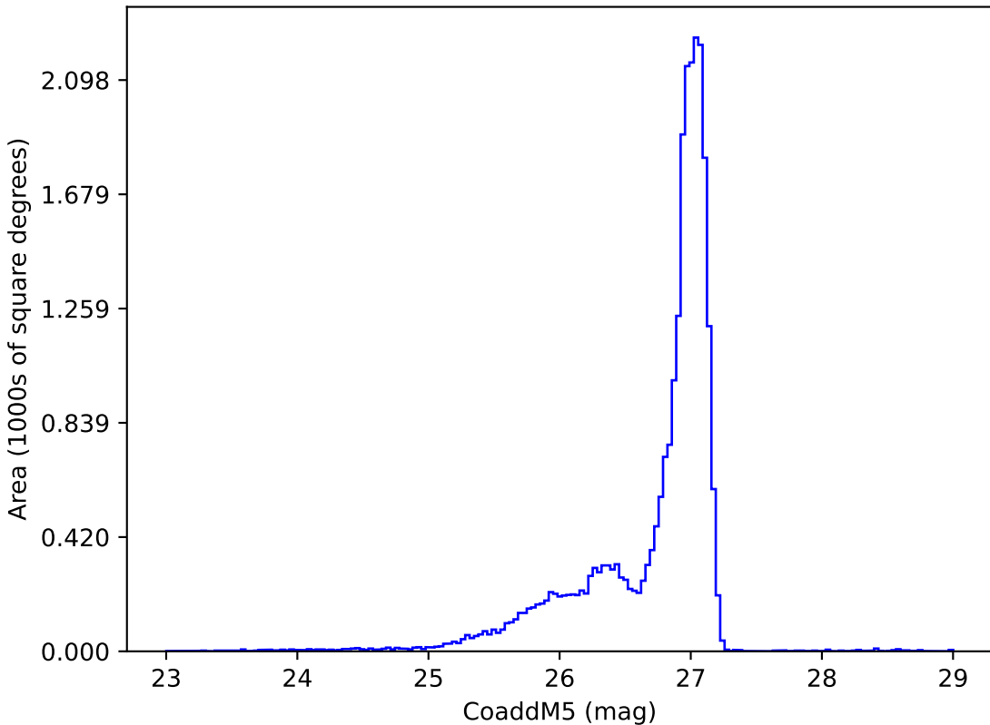
ddf_acor_sf15_lsf40_lsr50_v3.4_10yrs r: CoaddM5
