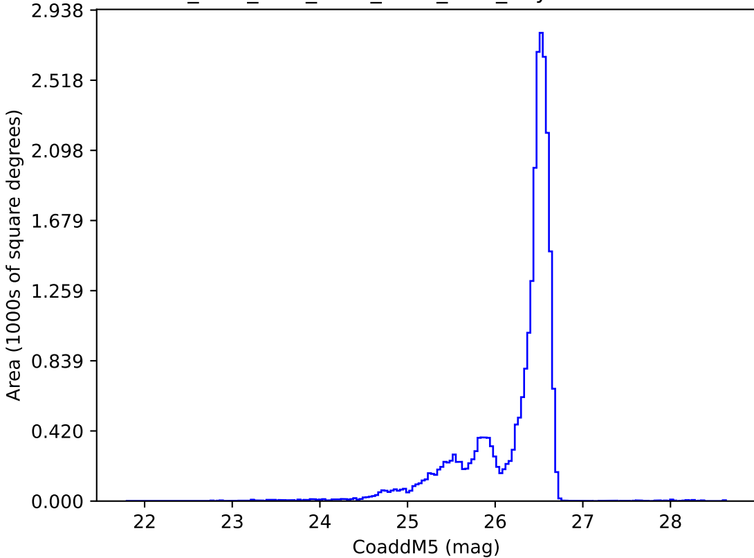
ddf_acor_sf15_lsf40_lsr50_v3.4_10yrs i: CoaddM5
