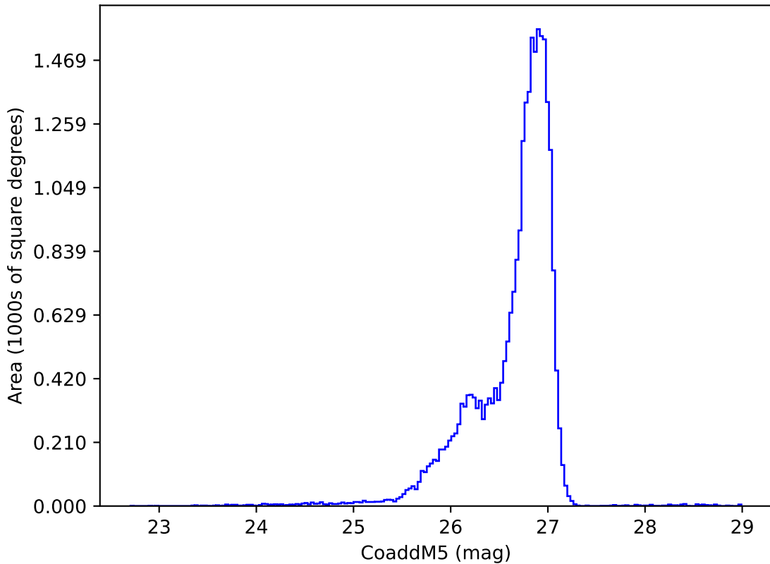
ddf_acor_sf15_lsf40_lsr50_v3.4_10yrs g: CoaddM5
