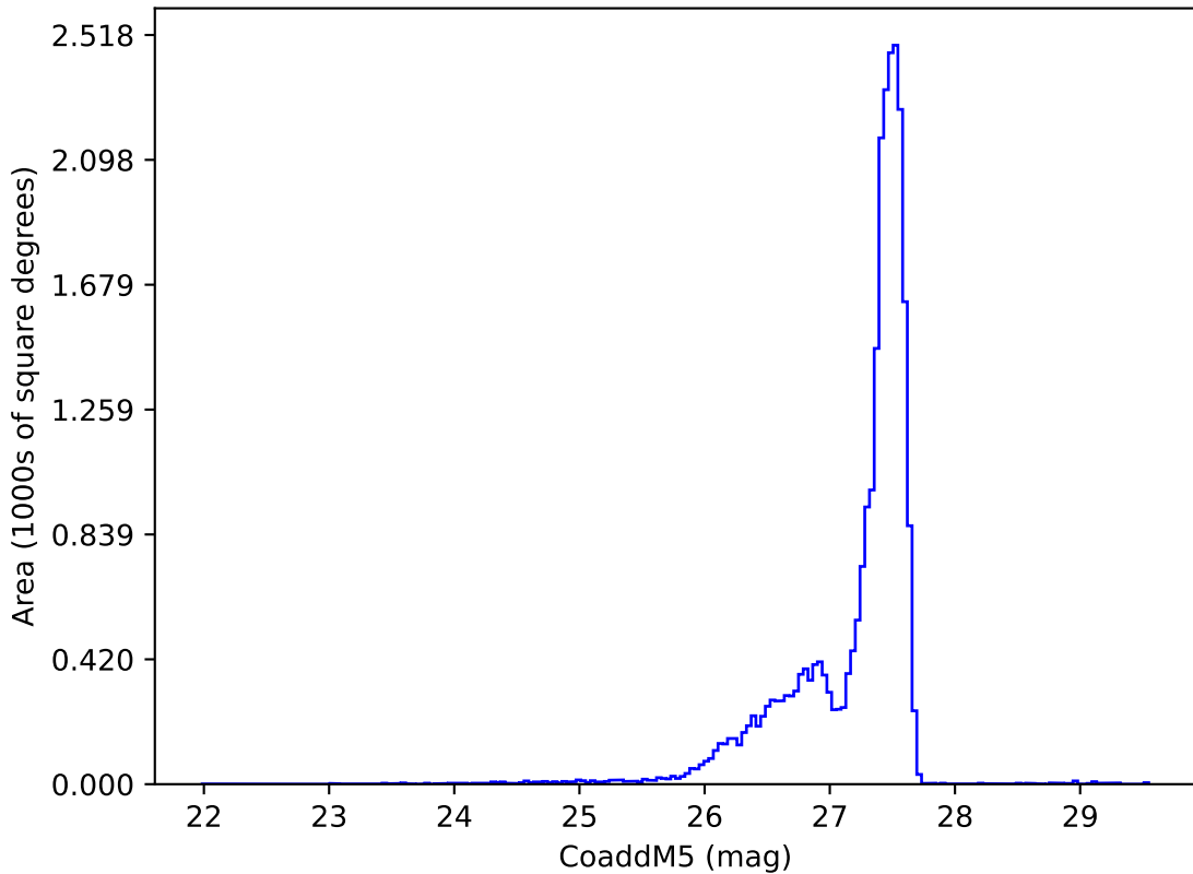
ddf_acor_sf15_lsf40_lsr50_v3.4_10yrs : CoaddM5
