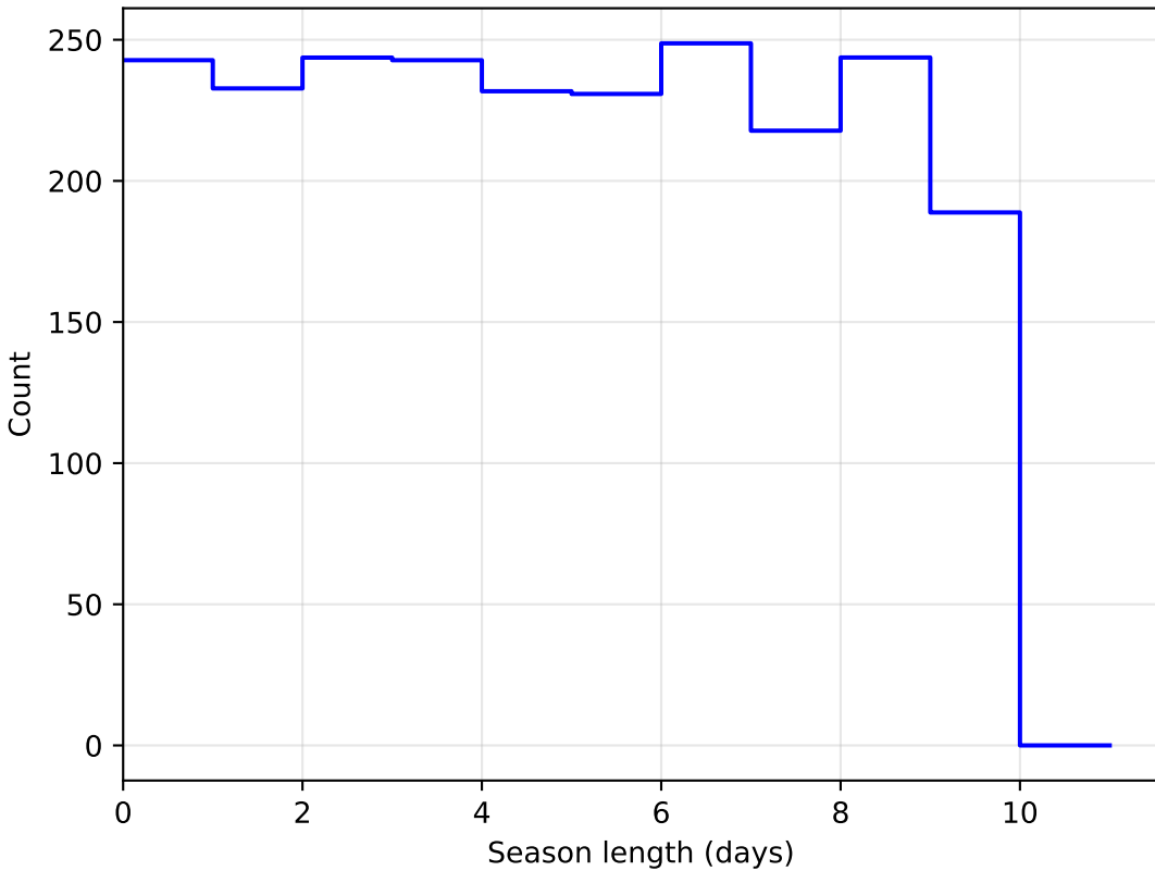
ddf_acor_sf15_lsf40_lsr50_v3.4_10yrs DD:EDFS all bands: SeasonLength
