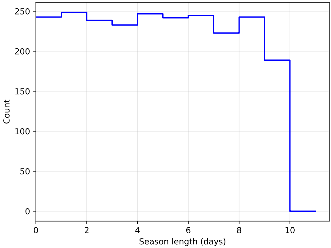
ddf_acor_sf15_lsf40_lsr50_v3.4_10yrs DD:ECDFS all bands: SeasonLength
