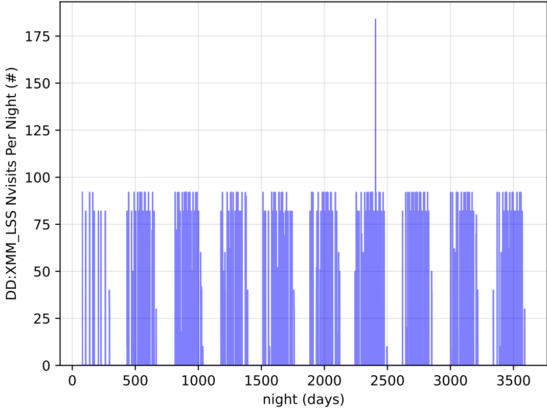
ddf_acor_sf15_ls40_lsr50_v3.4_10yrs all bands: DD:XMM_LSS Nvisits Per Night
