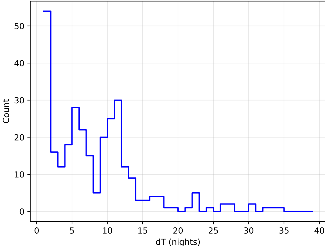
ddf_acor_sf15_lsf40_lsr50_v3.4_10yrs all bands: DD:XMM_LSS Delta Nights Histogram
