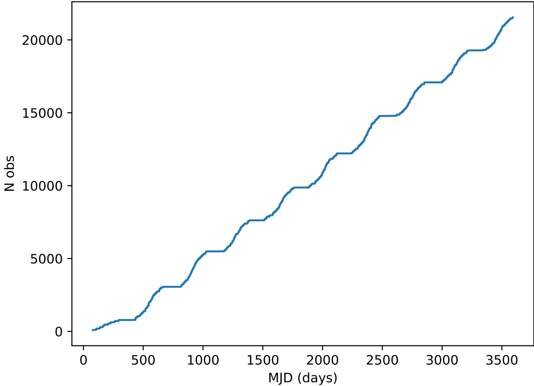
ddf_acor_sf15_lsf40_lsr50_v3.4_10yrs all bands: DD:XMM_LSS Cumulative NVisits
