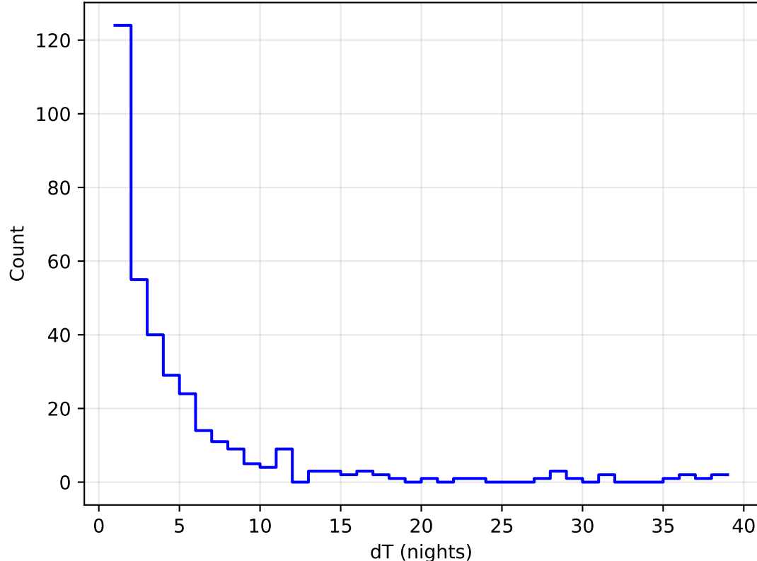
ddf_acor_sf15_lsf40_lsr50_v3.4_10yrs all bands: DD:WFD Delta Nights Histogram
