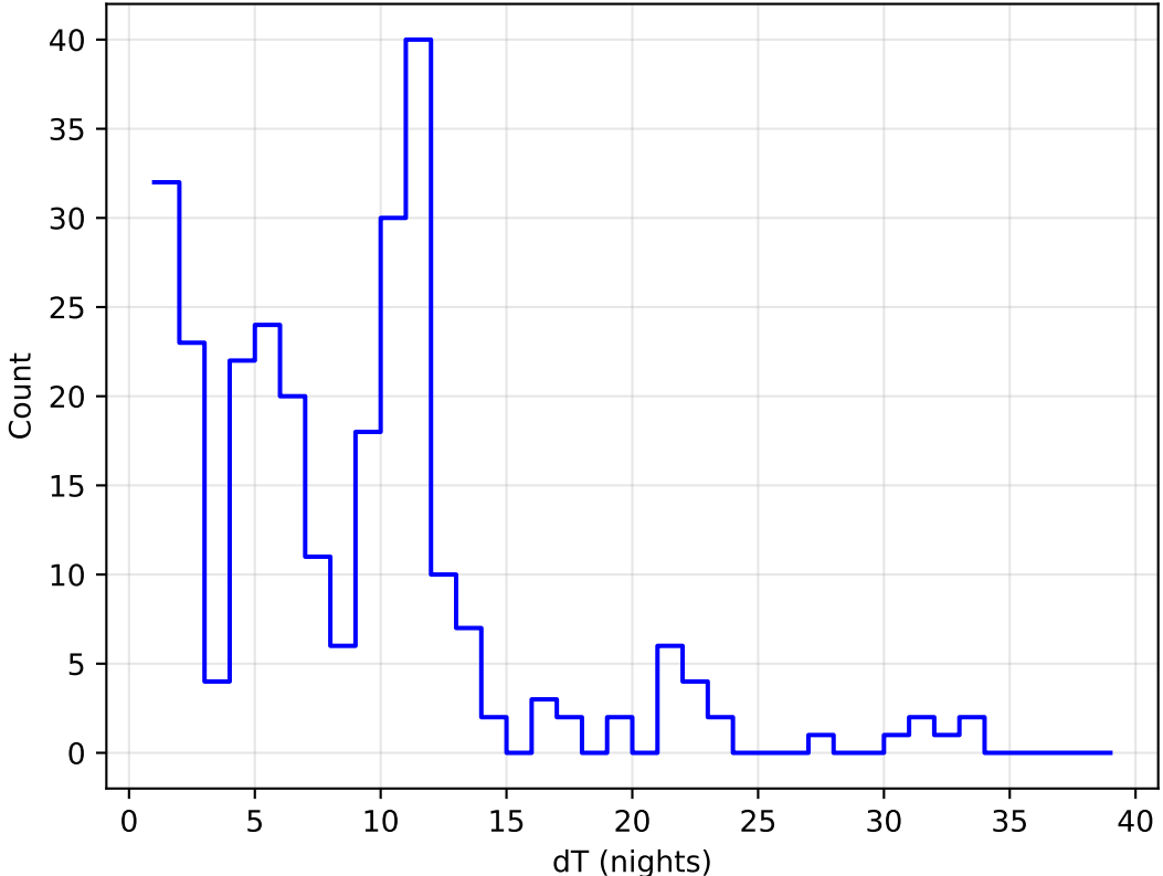
ddf_acor_sf15_lsf40_lsr50_v3.4_10yrs all bands: DD:ELAISS1 Delta Nights Histogram
