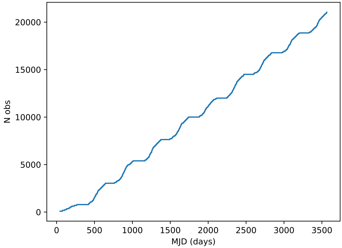
ddf_acor_sf15_lsf40_lsr50_v3.4_10yrs all bands: DD:ELAISS1 Cumulative NVisits
