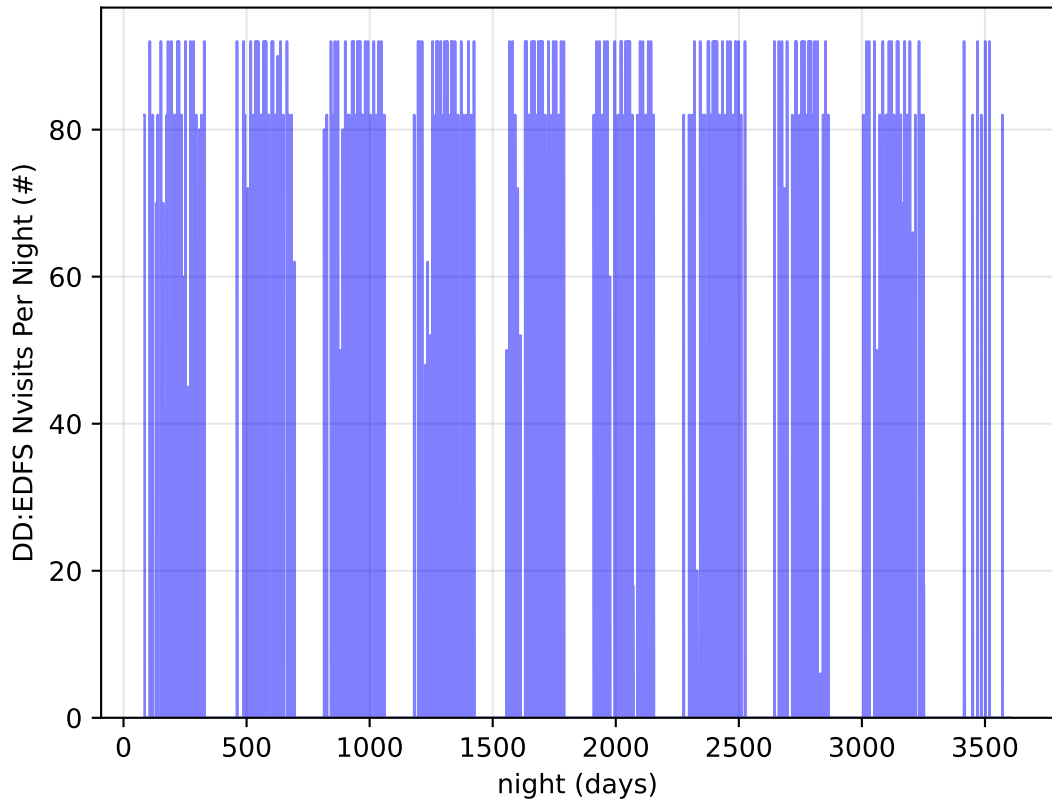
ddf_acor_sf15_lsf40_lsr50_v3.4_10yrs all bands: DD:EDFS Nvisits Per Night
