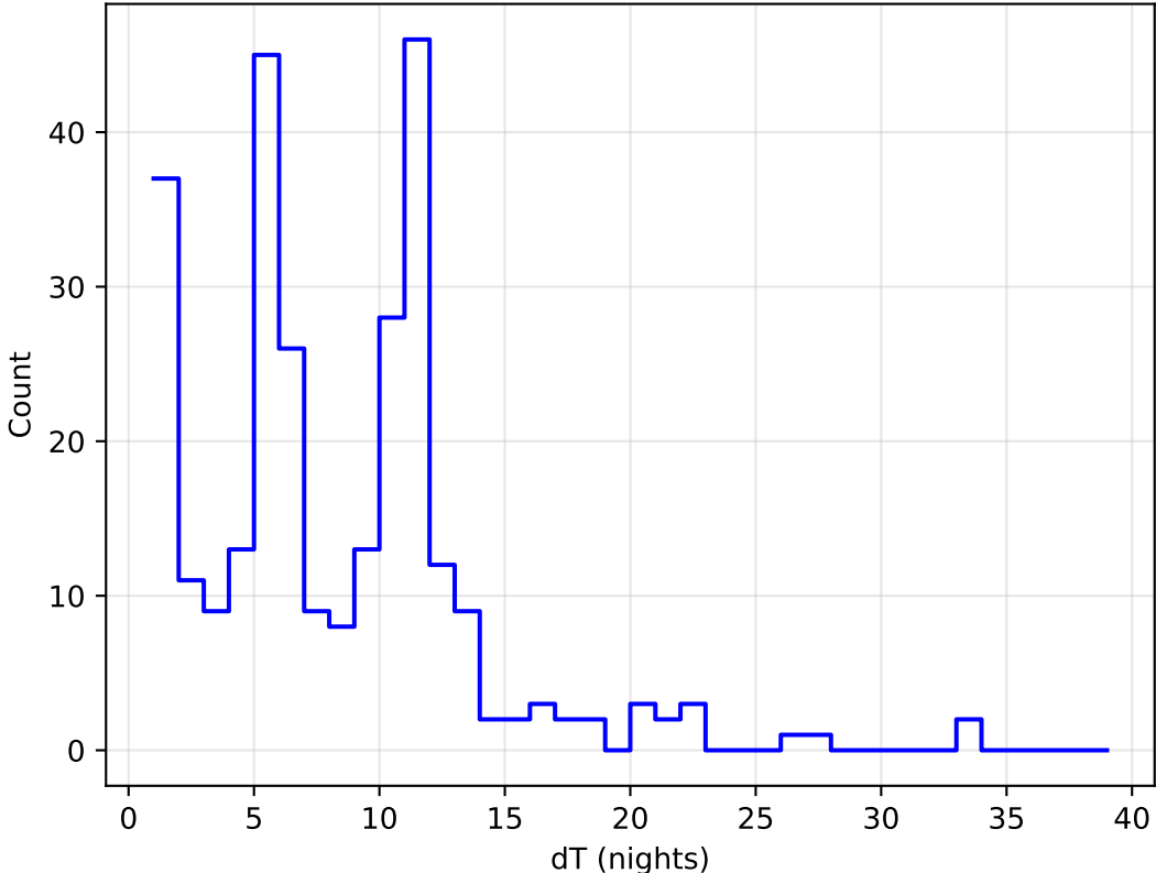
ddf_acor_sf15_lsf40_lsr50_v3.4_10yrs all bands: DD:EDFS Delta Nights Histogram
