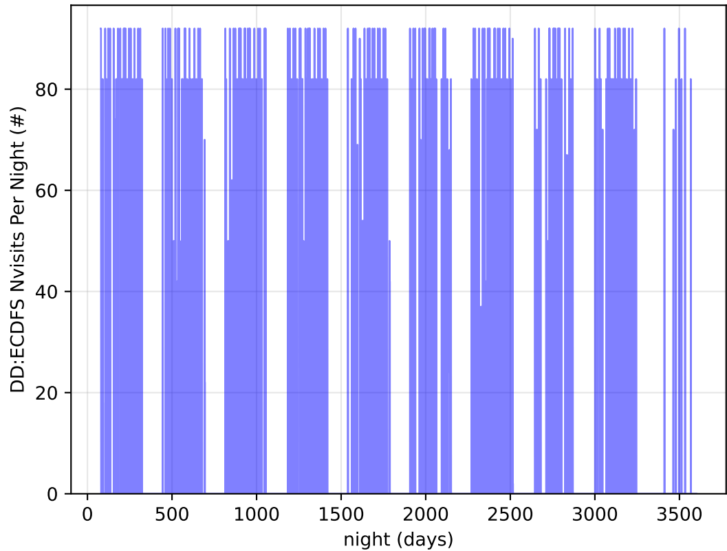
ddf_acor_sf15_lsf40_lsr50_v3.4_10yrs all bands: DD:ECDFS Nvisits Per Night
