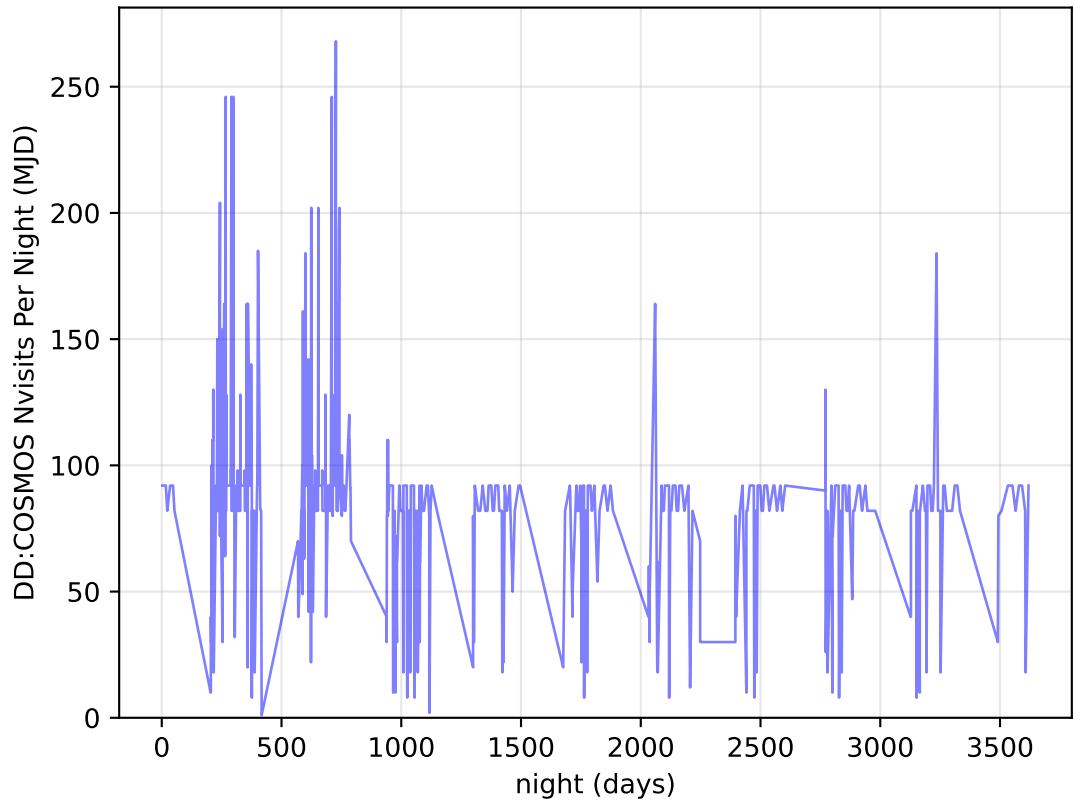
ddf_acor_sf15_lsf40_lsr50_v3.4_10yrs all bands: DD:COSMOS Nvisits Per Night
