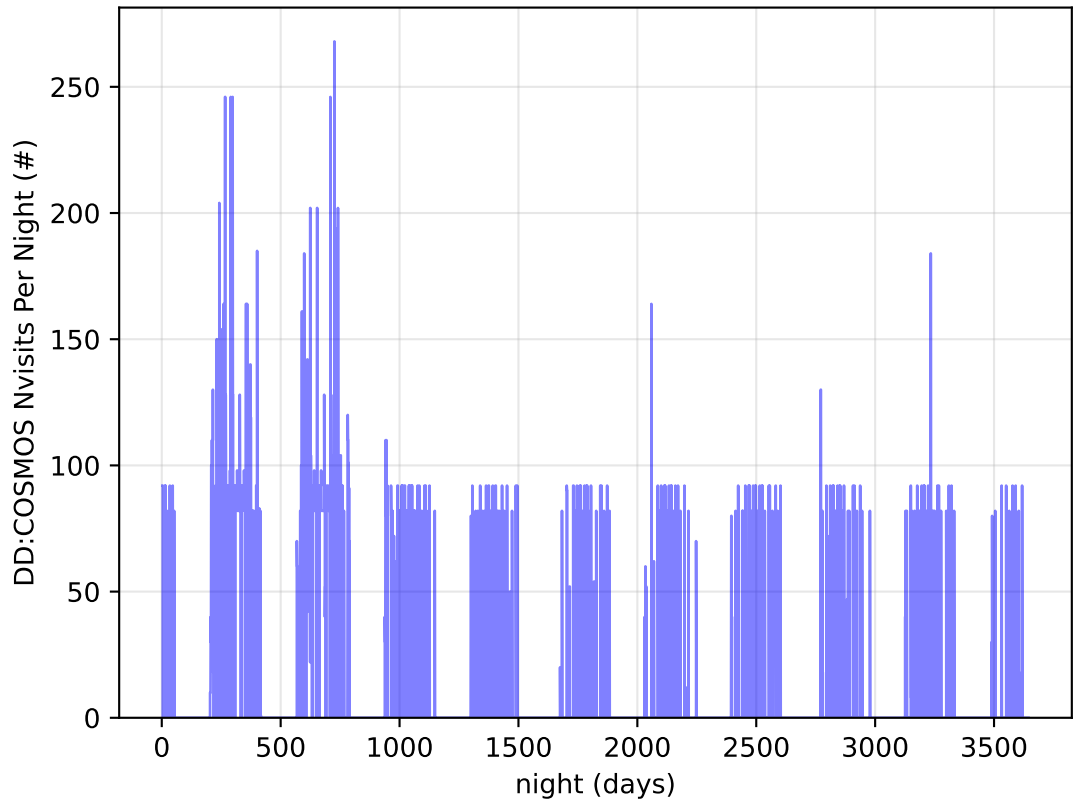
ddf_acor_sf15_lsf40_lsr50_v3.4_10yrs all bands: DD: COSMOS Nvisits Per Night
